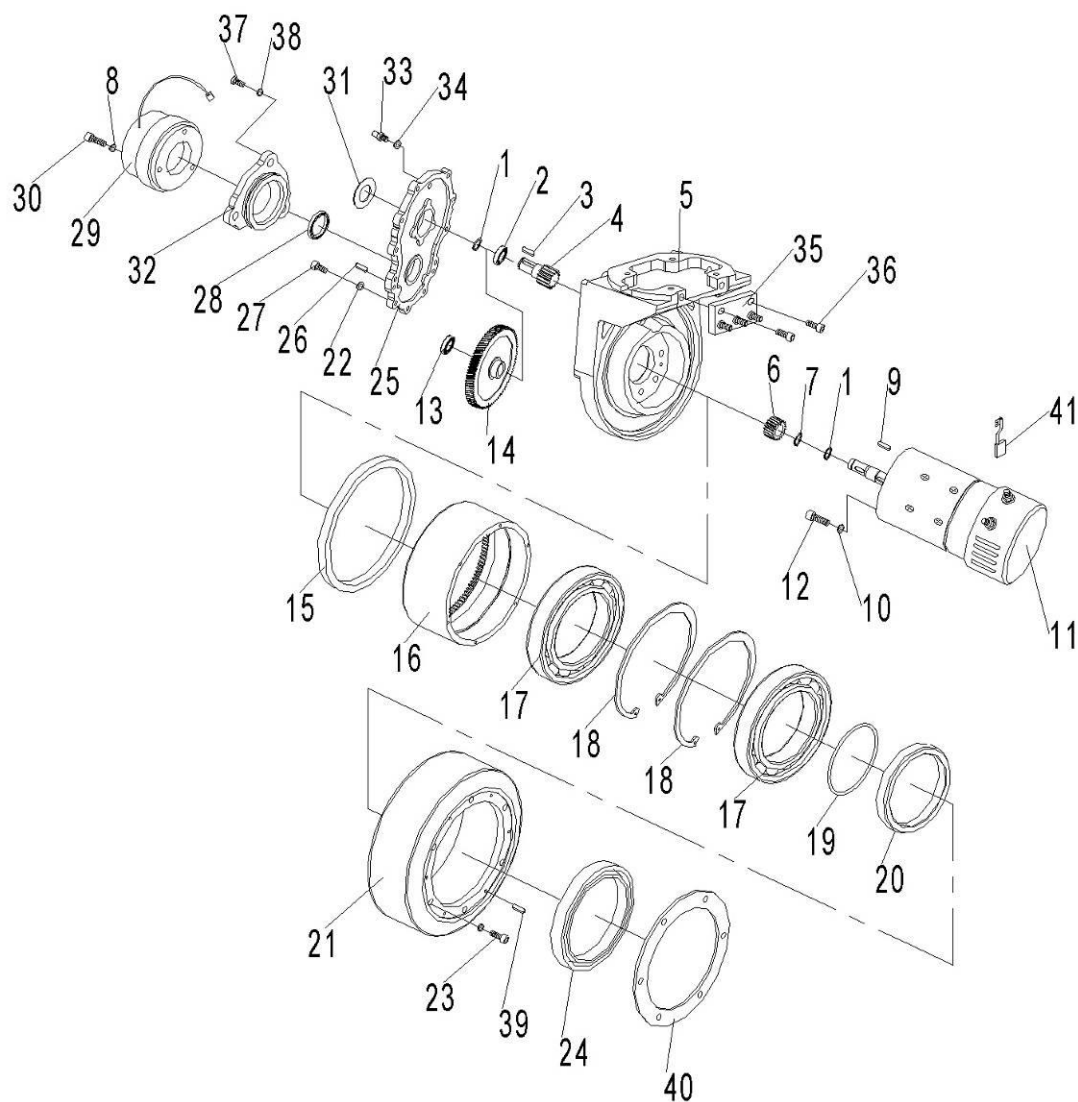
Fig. 5 Drive wheel
