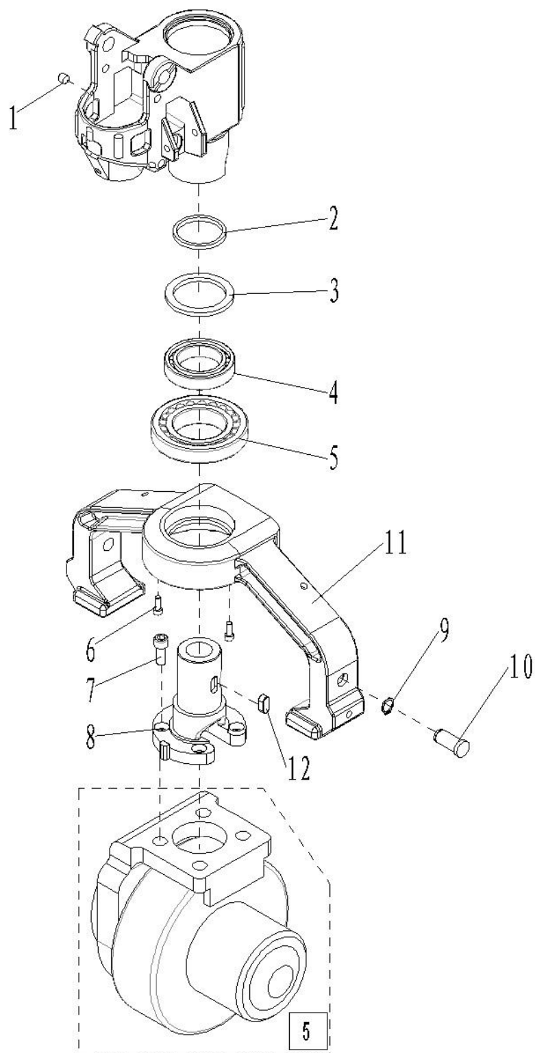
Fig. 3 Drive system
