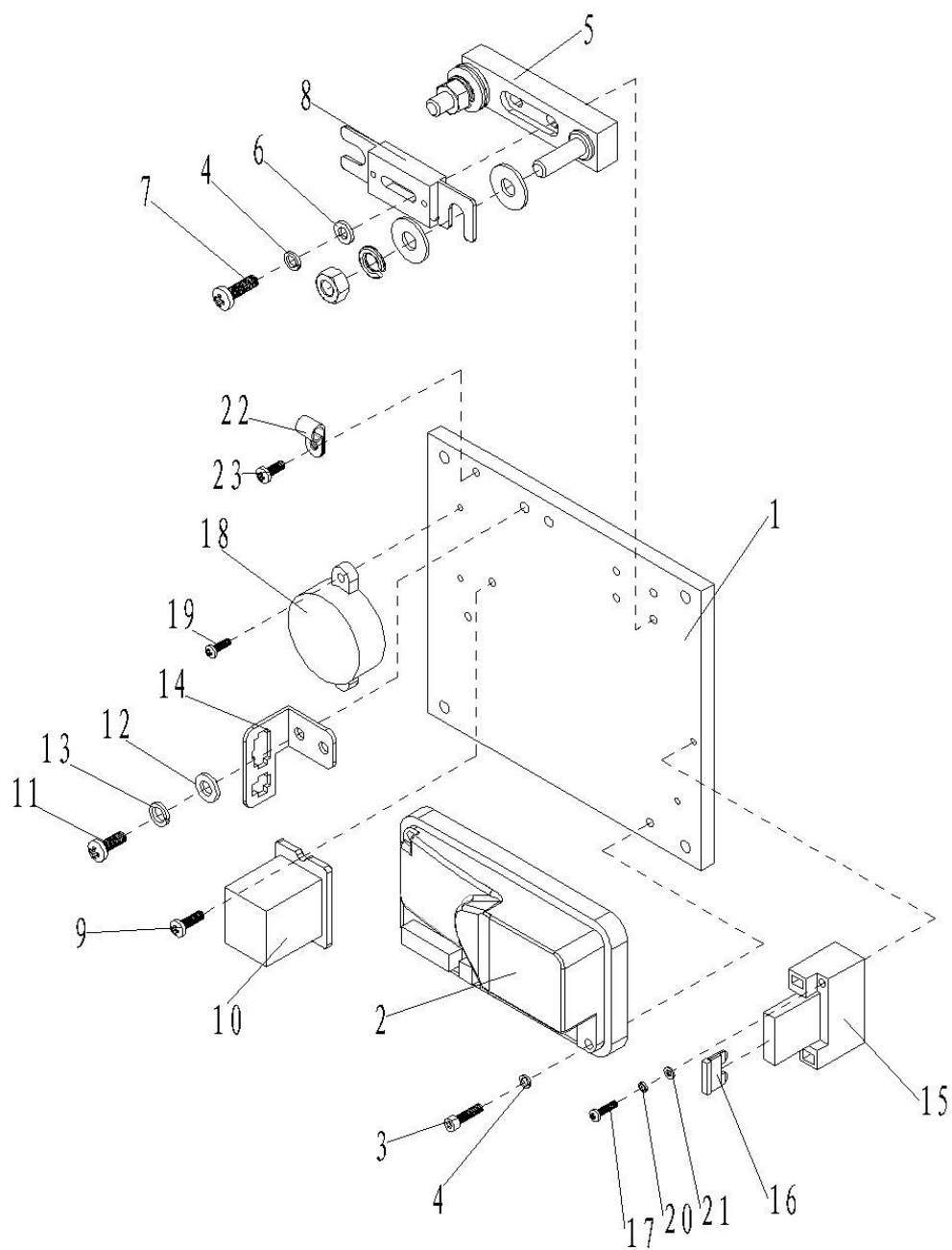
Fig. 10 Control system
